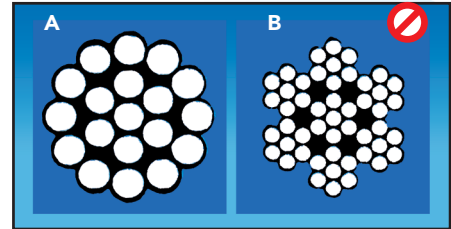
Python Standard
